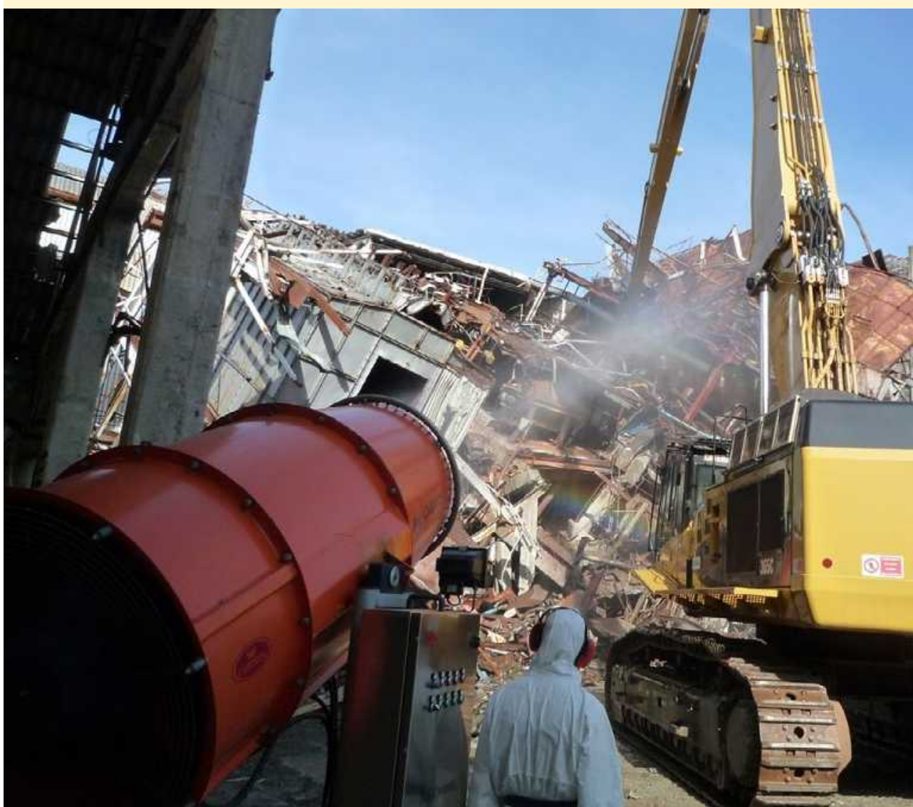
Figure 15-8: Nebulising cannon to dampen dust during demolition of a production plant
