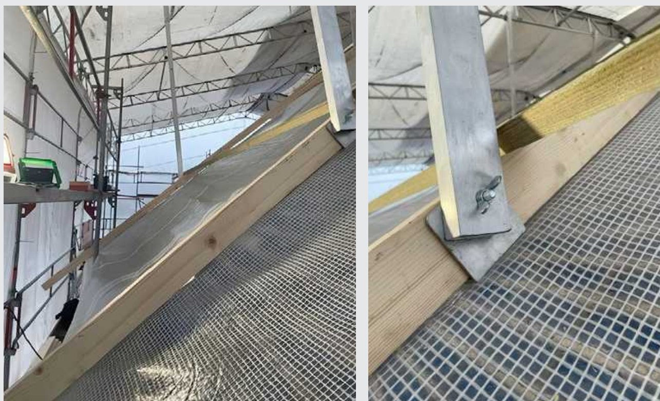
Figure 13-4: Suspension system inside an asbestos tent
